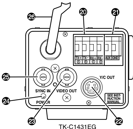
TK-C1431EG
